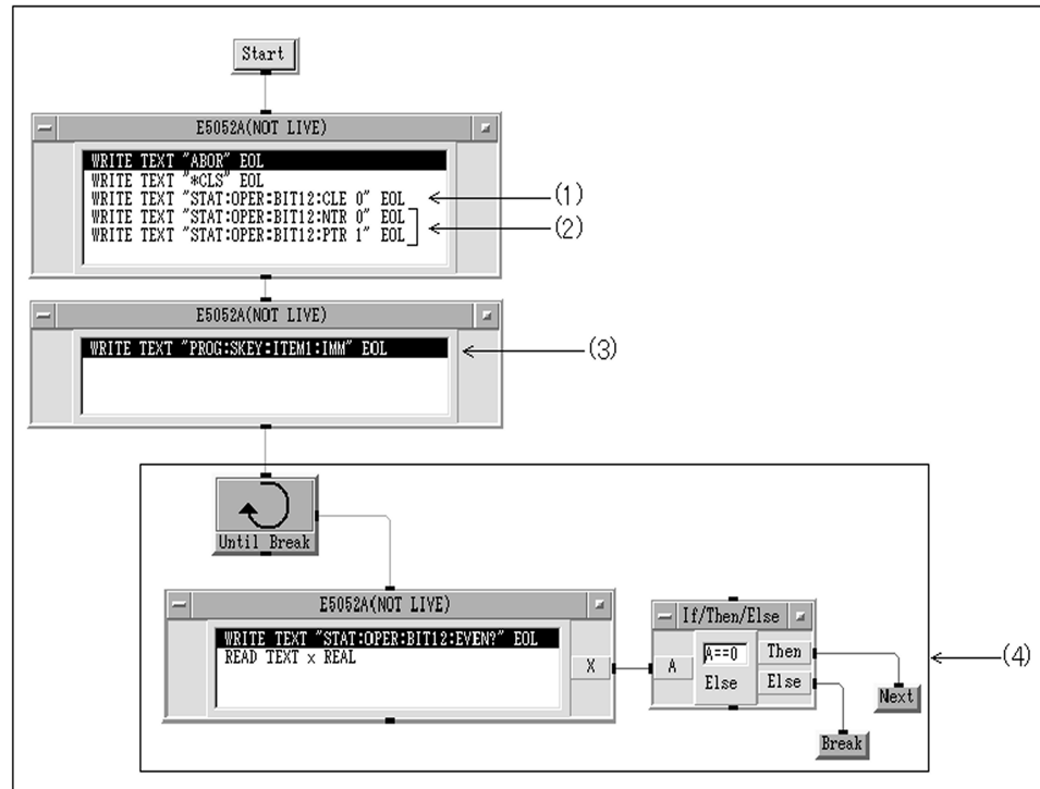
Figure 4-3 A Sample Program to Control User-defined Register (On the Controller Side)
